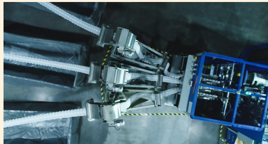
Pocketed spring units manufacturing
